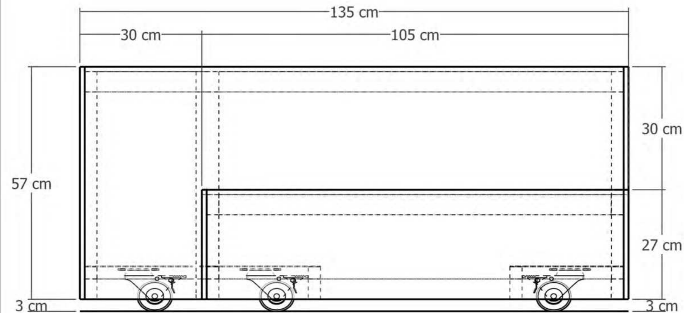
Vista Frontal
